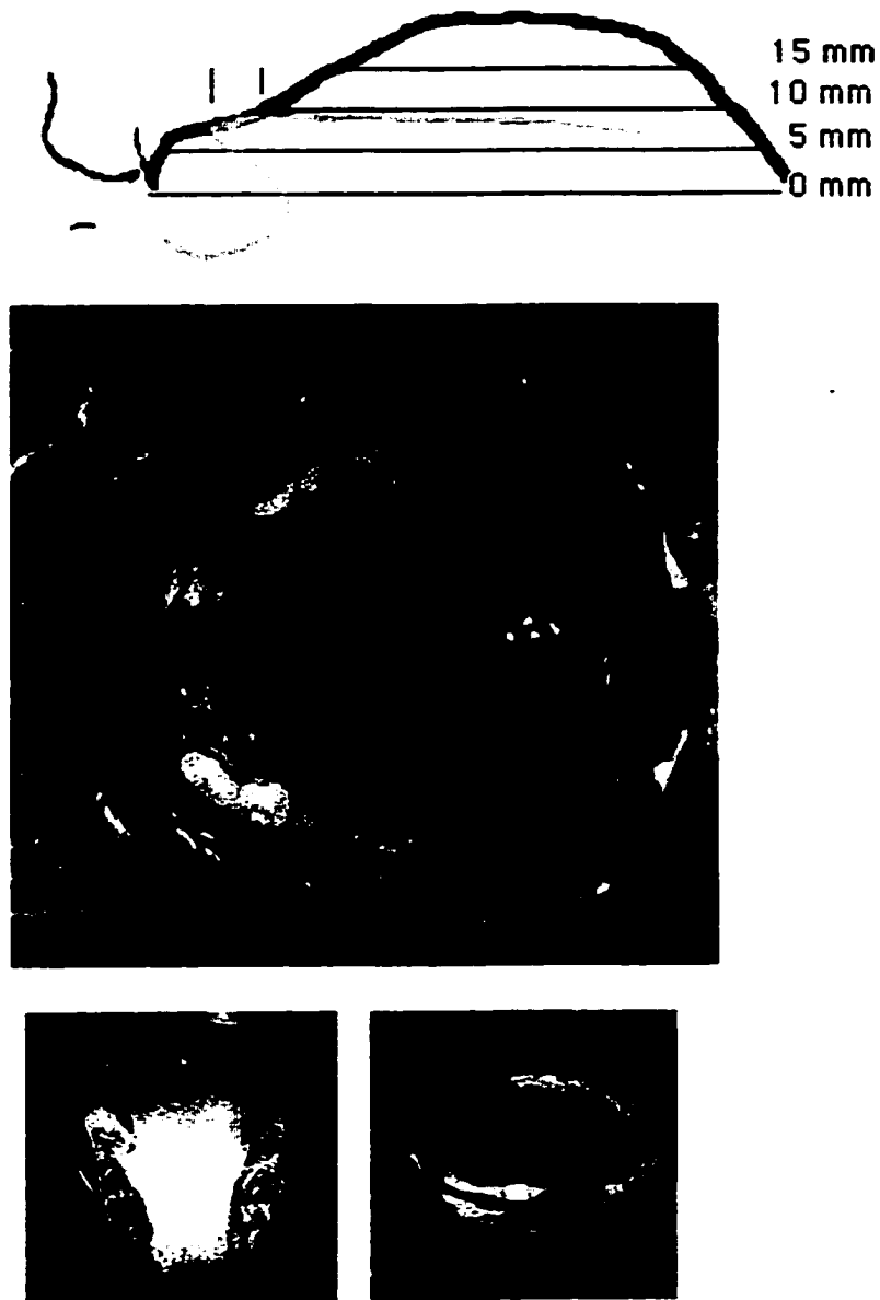
Figure 3.57: Palatogram, linguograms and reconstructed midsagittal section for a stop which is phonologically [+apical] and non-contrastive for Anterior. Articulation: apical alveolar. Token: /'Təpə/ back (n.)
