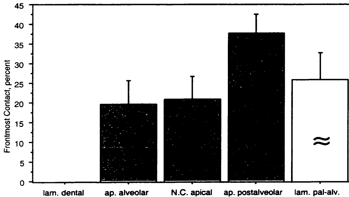
Figure 3.47: Frontmost contact in percent for coronal Place categories
