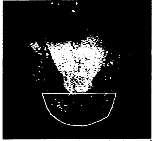
Figure 3.36b: Categorization of linguograms according to shape : 'triangle'.
