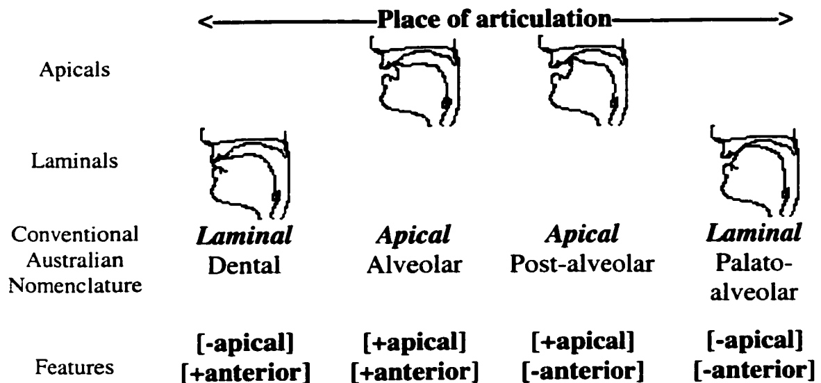
Figure 1.5: Impressionistically-based descriptions of tongue configurations for W. Arrernte coronals
