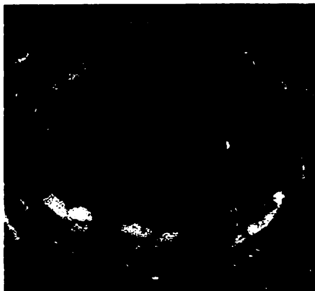
Figure 3.60: Palatogram and reconstructed midsagittal section for a phonologically [-apical] [+anterior] stop. The interdental linguogram is not available. Articulation: laminal interdental. Token: /'pəʔə/ pouch (n.)
