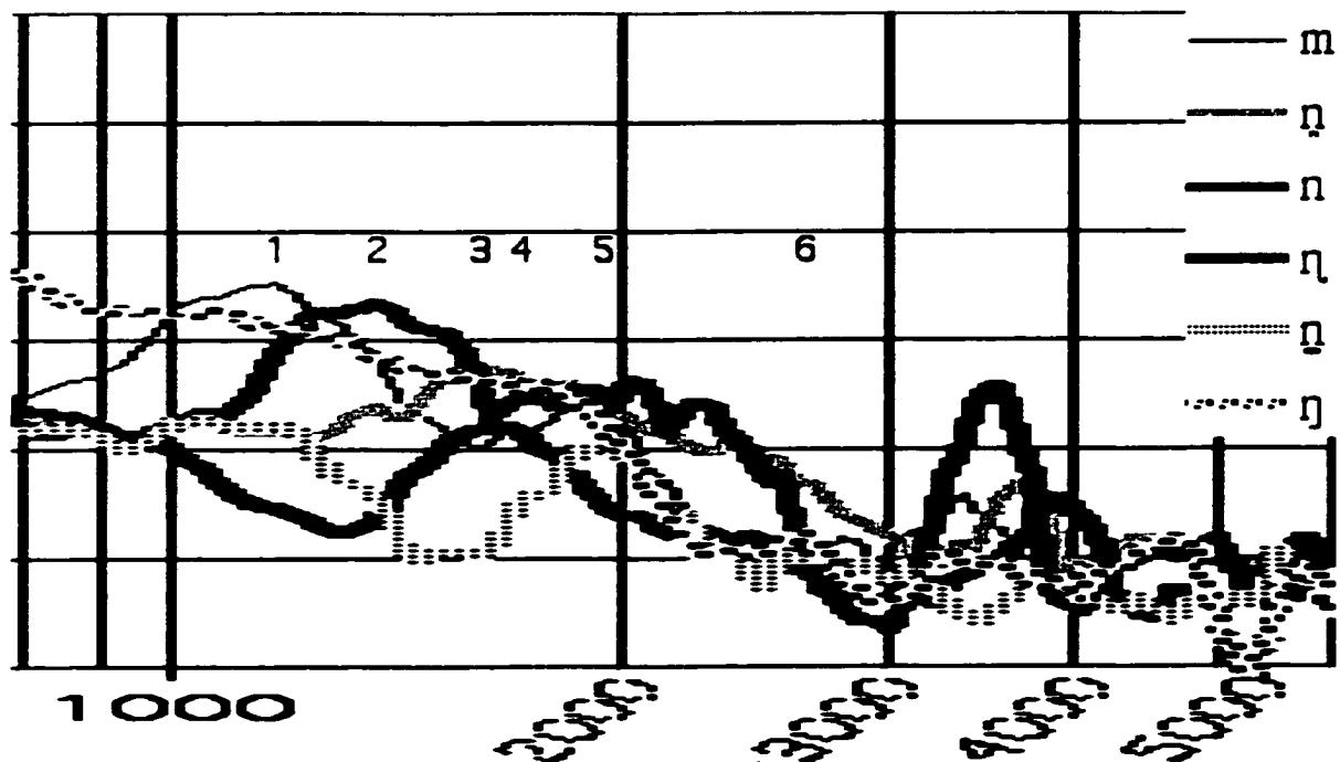
Figure 4.13b: Male speaker's nasal murmur spectra, 1000-5000 Hz. Numbers are vertically aligned with peaks discussed in the text.
