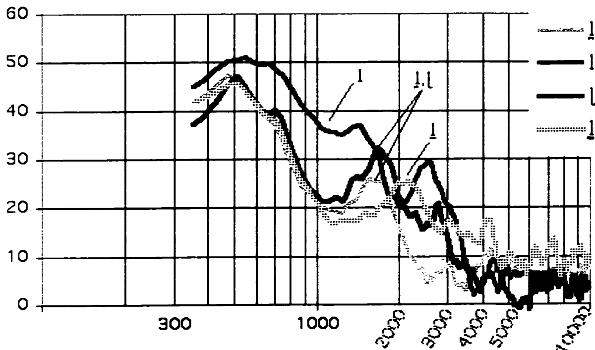
Figure 4.16a: Female speaker's lateral murmur spectra, 100-10000 Hz.
