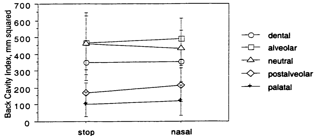
Figure 3.42: Back cavity index in millimeters for coronal Place categories: stops versus nasals ( p=.4848 .)
