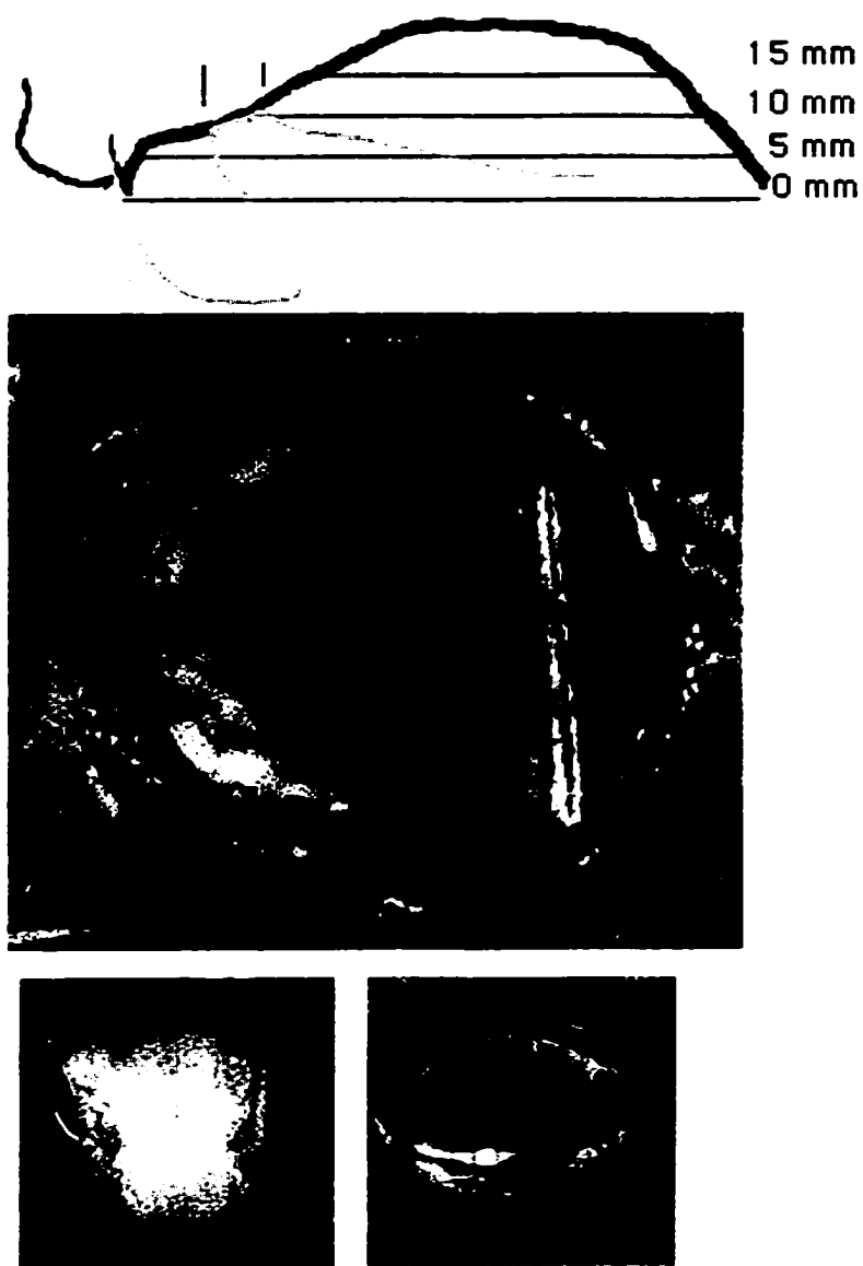
Figure 3.58: Palatogram, linguograms and reconstructed midsagittal section for a phonologically [+apical] [-anterior] nasal. Articulation: sublaminal alveolar or postalveolar. Token: /'mənə/ veg. food (n.)
