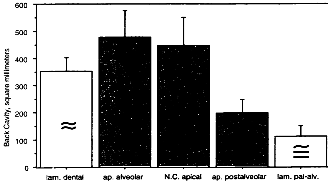
Figure 3.50: Back cavity index in millimeters for coronal Place categories
