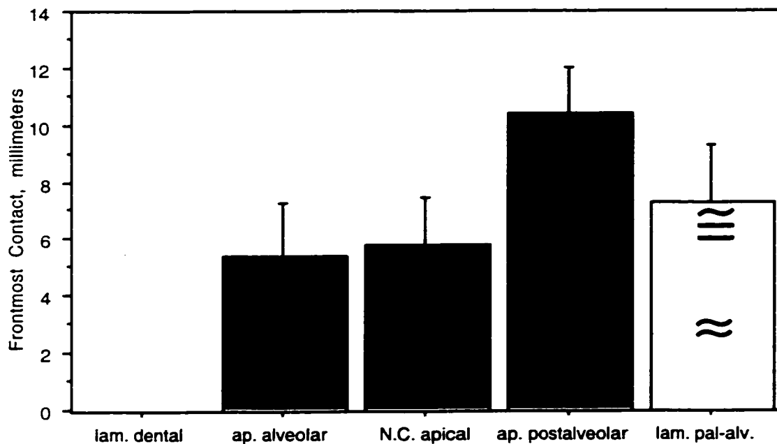
Figure 3.46: Frontmost contact in millimeters for coronal Place categories
