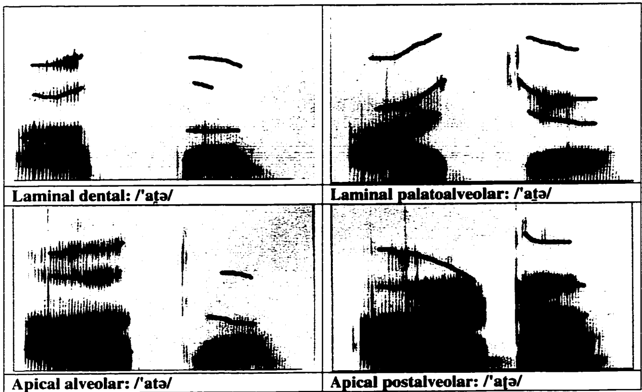
Figure 4.10: Spectrograms of four stop tokens for one speaker with formant tracings added.
