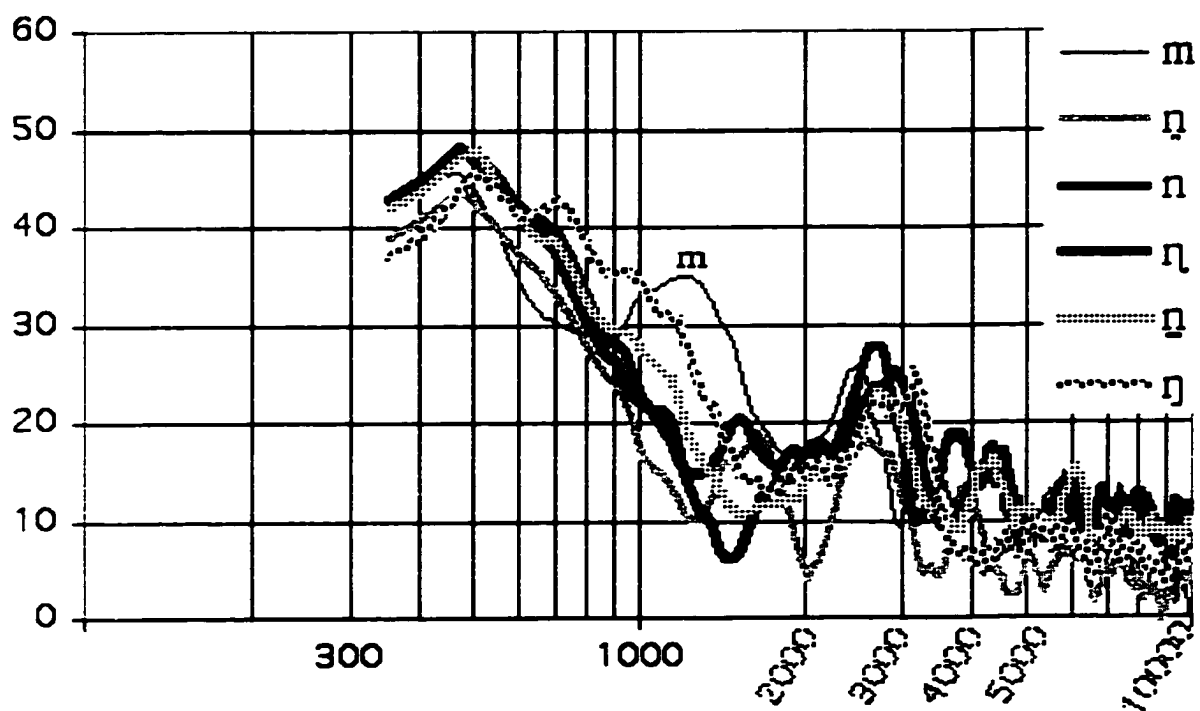
Figure 4.14a: Female speaker's nasal murmur spectra, 100-10000 Hz.
