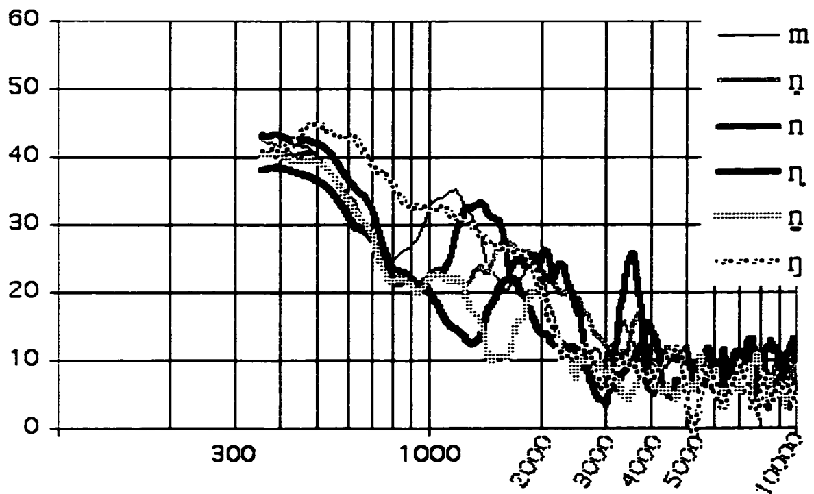
Figure 4.13a: Male speaker's nasal murmur spectra, 100-10000 Hz.
