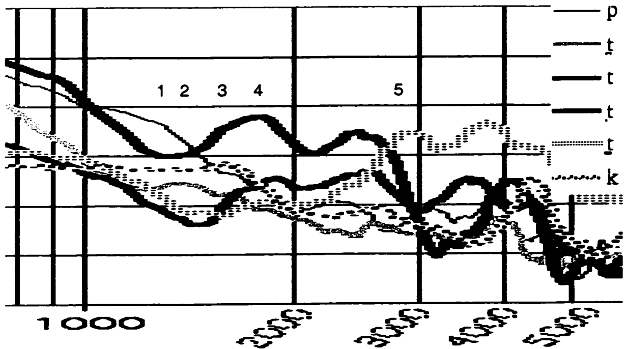
Figure 4.12b: Female speaker's stop burst spectra, 1000-5000 Hz. Numbers are vertically aligned with peaks discussed in the text.
