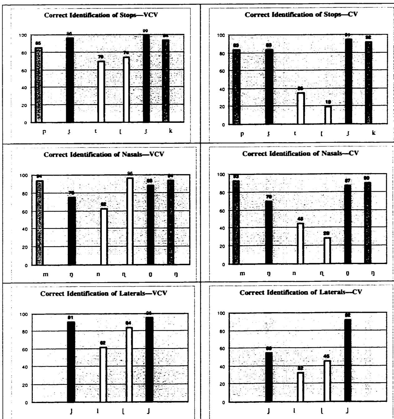
Figure 4.7: Rates of correct identification of stops, nasals and laterals. VCV responses are shown at left; CV responses at right.
