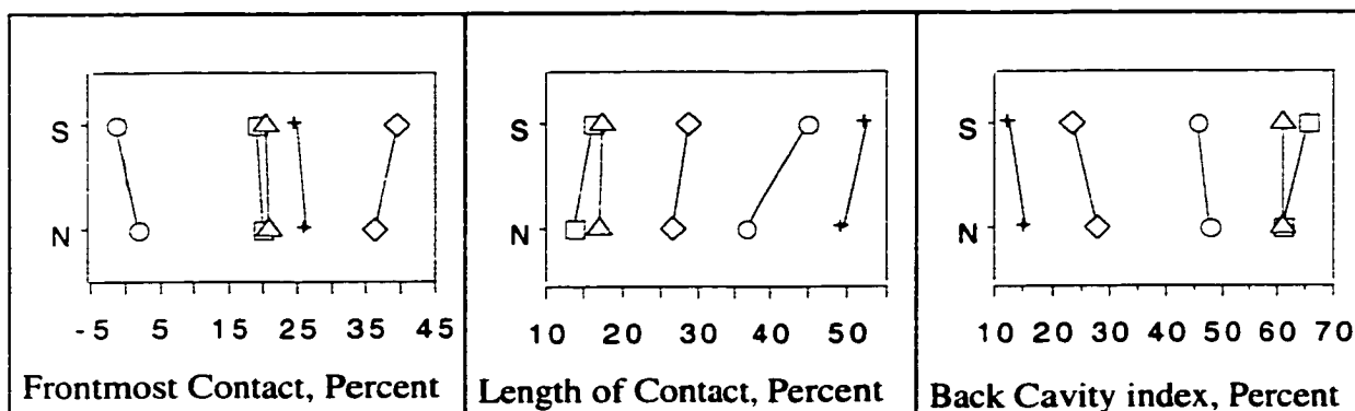
Figure 3.44: Summary of results: stops (top rows) versus nasals (bottom rows.)
