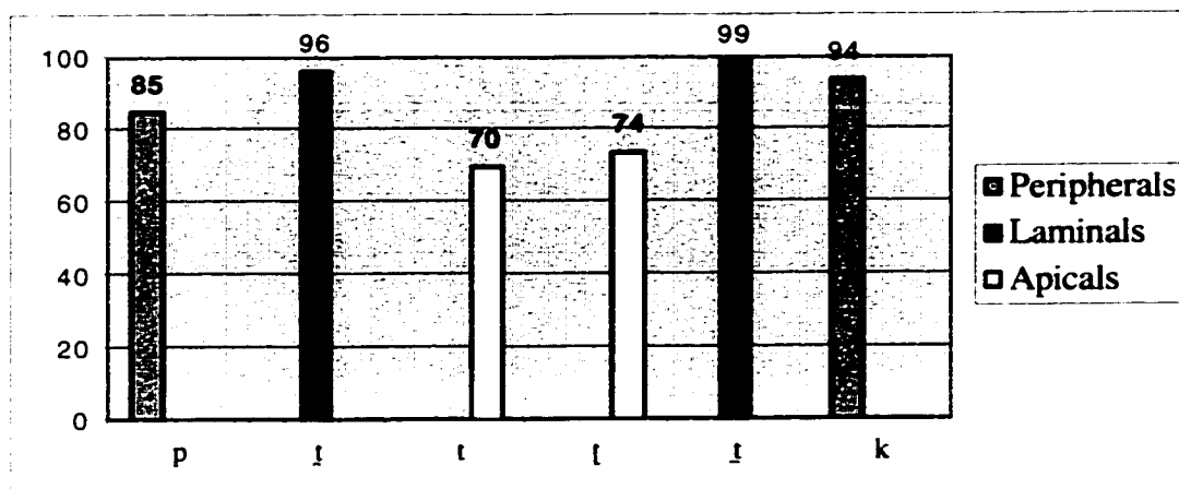
Figure 4.2a: Percent correct identification of stops—VCV condition
