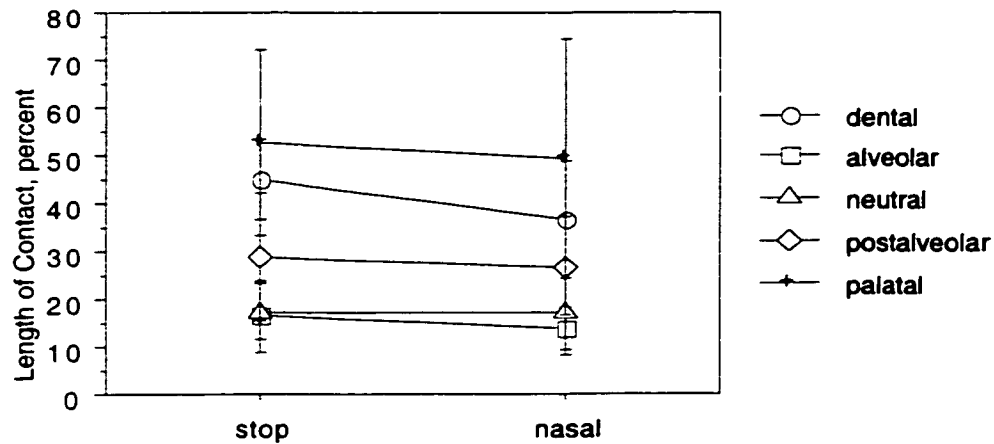
Figure 3.41: Length of contact in percent for coronal Place categories: stops versus nasals ( p=.0901 .)
