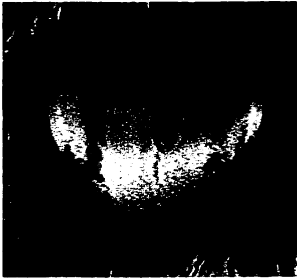
Figure 3.33a: Categorization of linguograms according to shape : 'parallel lines.' Upper surface of tongue.
