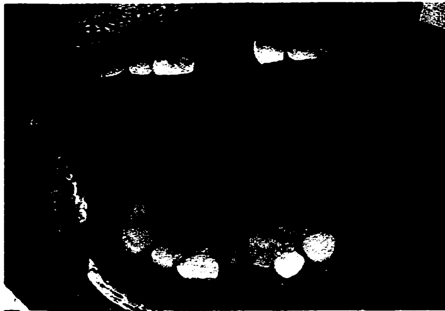
Figure 3.3: Palatogram; still image digitized from video. Orientation: Upper teeth shown at top and reflected in the mirror at bottom. Token: /pətə/ 'rock'.
