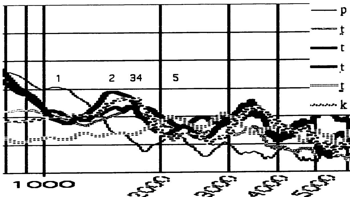
Figure 4.11b: Male speaker's stop burst spectra, 1000-5000 Hz. Numbers are vertically aligned with peaks discussed in the text.
