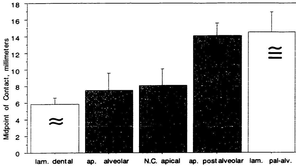
Figure 3.52: Midpoint of Contact in millimeters for coronal Place categories
