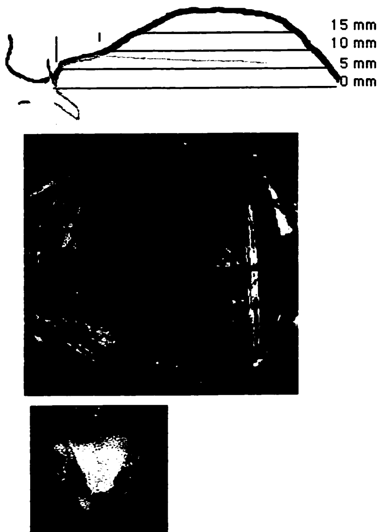
Figure 3.59: Palatogram, linguogram and reconstructed midsagittal section for a phonologically [-apical] [+anterior] stop. Articulation: apicolaminal dentalalveolar. Token: /'təmə/ grind (vt)
