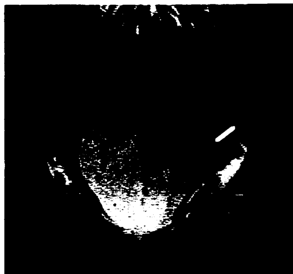
Figure 3.32: Categorization of linguograms according to coronal width at tongue front: 'narrow.' Note that the illustration line is shown at an angle, to reflect the cupped position of the tongue in this frame.
