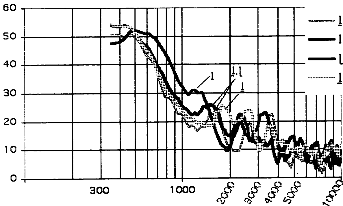
Figure 4.15a: Male speaker's lateral murmur spectra, 100-10000 Hz.
