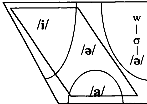
Figure 2.2: Author's impressionistic vowel space for W. Arernte. The parallelogram shows the allophonic range of unrounded /ə/, while the high back area shows the range for rounded /ə/.
