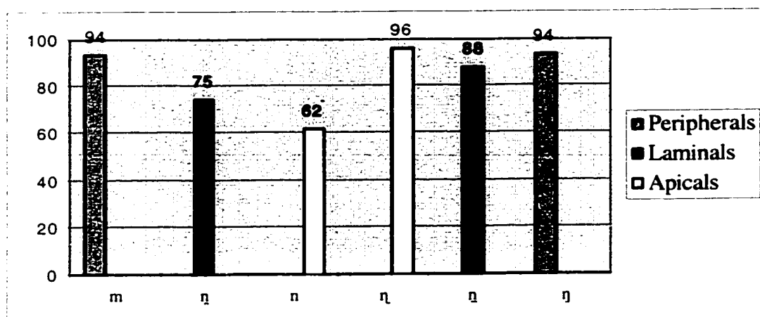
Figure 4.2b: Percent correct identification of nasals—VCV condition
