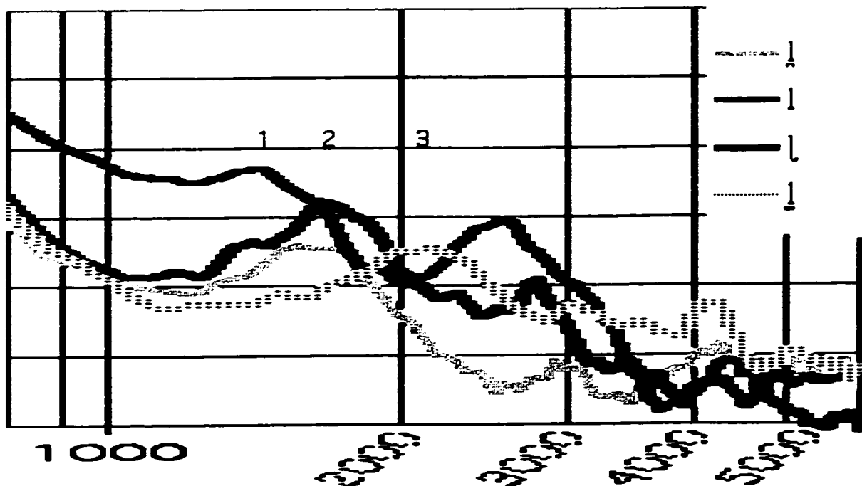
Figure 4.16b: Female speaker's lateral murmur spectra, 1000-5000 Hz. Numbers are vertically aligned with peaks discussed in the text.
