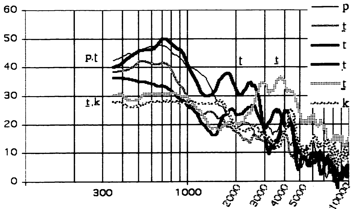
Figure 4.12a: Female speaker's stop burst spectra, 100-10000 Hz.
