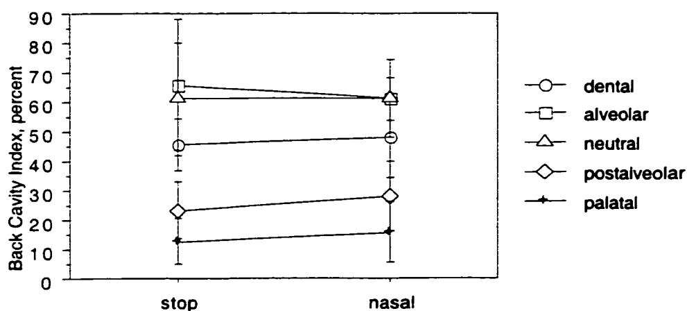
Figure 3.43: Back cavity index in percent for coronal Place categories: stops versus nasals ( p=.4777 .)
