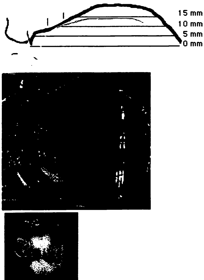
Figure 3.61: Palatogram, linguogram and reconstructed midsagittal section for a phonologically [-apical] [-anterior] stop. Articulation: laminal postalveolar. Token: /'petəmə/ is coming(vi)
