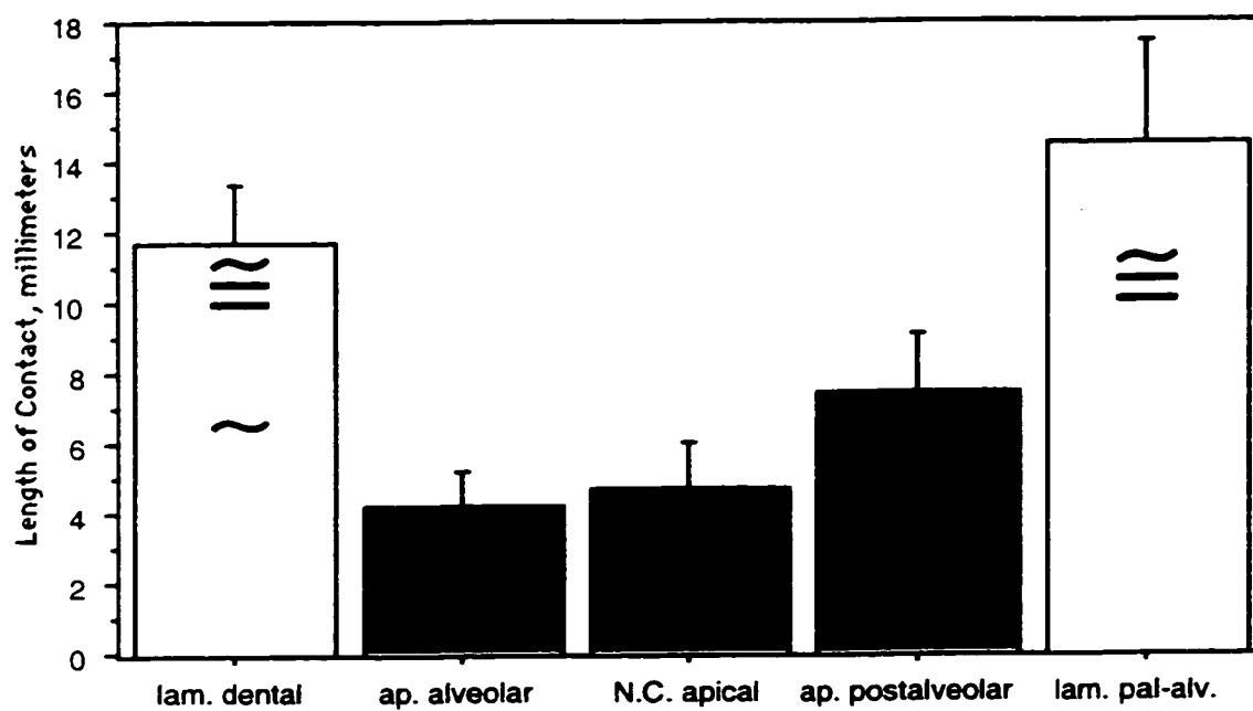
Figure 3.48: Length of contact in millimeters for coronal Place categories
