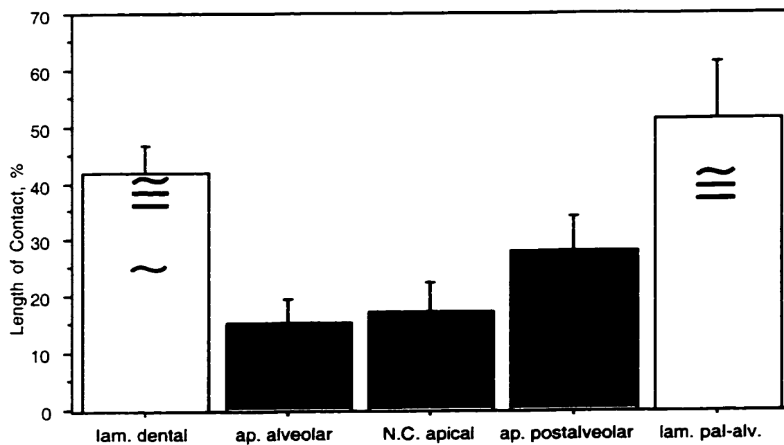
Figure 3.49: Length of contact in percent for coronal Place categories
