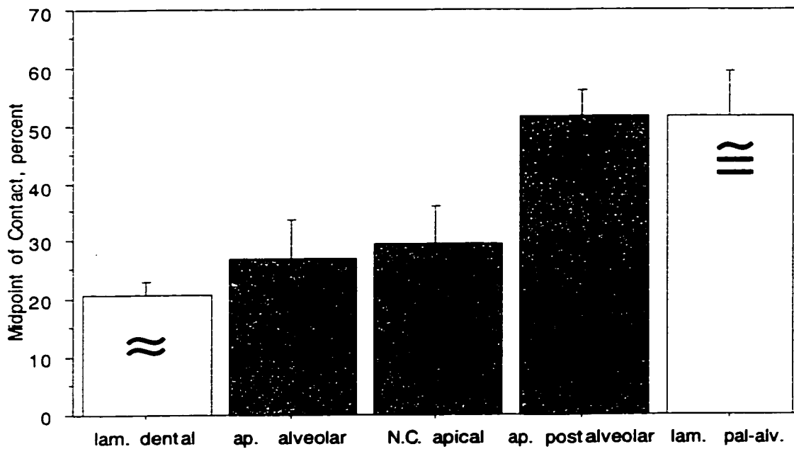
Figure 3.53: Midpoint of Contact in percent for coronal Place categories
