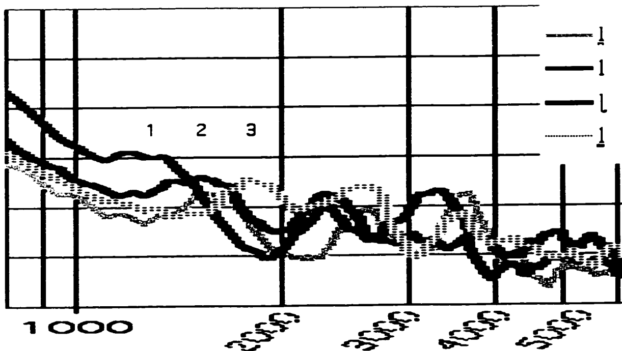
Figure 4.15b: Male speaker's lateral murmur spectra, 1000-5000 Hz. Numbers are vertically aligned with peaks discussed in the text.
