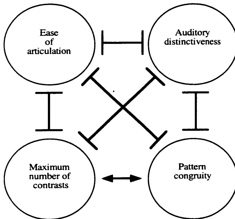
Figure 1.1: Relationships among four meta-principles governing linguistic sound structures. The double-headed arrow links the “harmonious” pair of principles; other pairings are likely to conflict.
