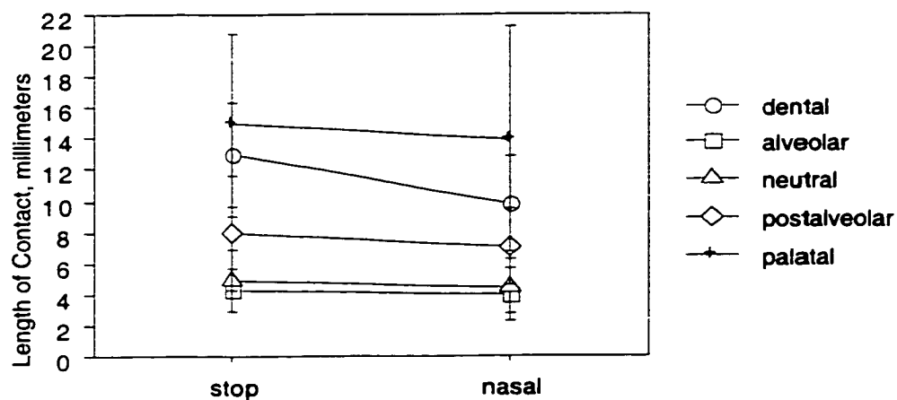
Figure 3.40: Length of contact in millimeters for coronal Place categories: stops versus nasals ( p=.0512 .)
