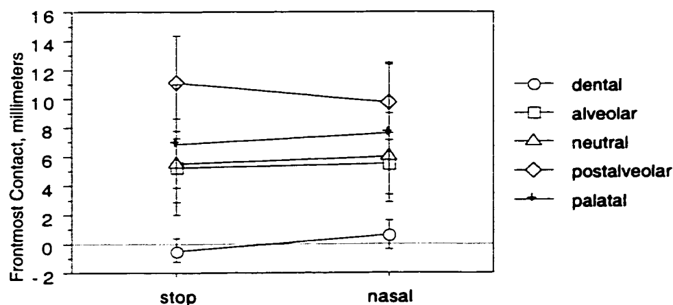
Figure 3.38: Frontmost contact in millimeters for coronal Place categories: stops versus nasals ( p = .1948 .)
