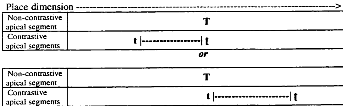
Figure 1.8a (top) and 1.8b (bottom): Arremte Gestural Economy Scenario--contrastive versus non-contrastive apicals
