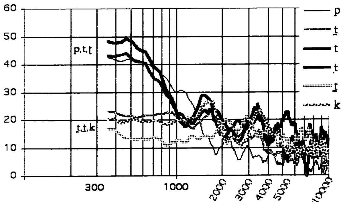
Figure 4.11a: Male speaker's stop burst spectra, 100-10000 Hz.
