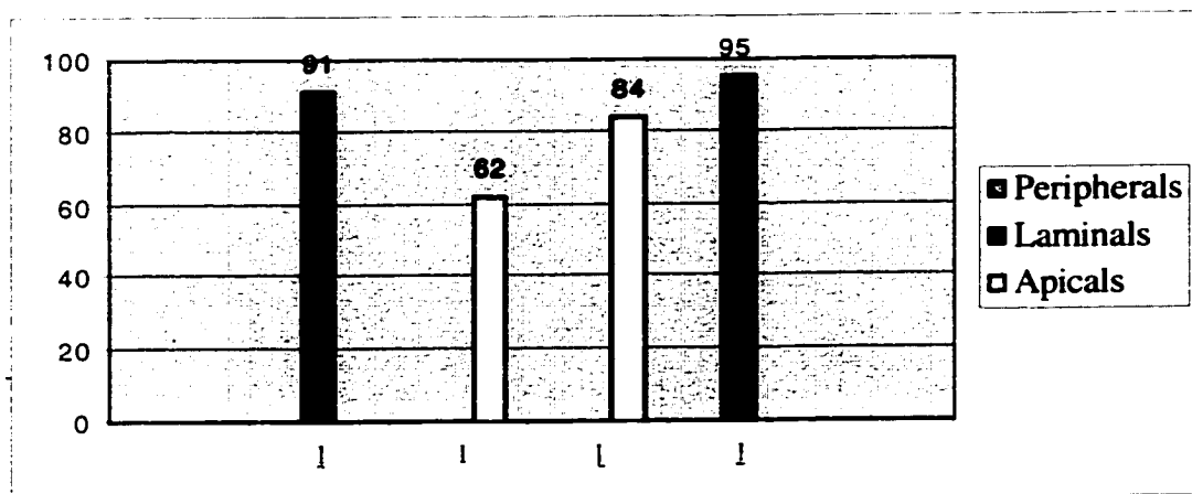
Figure 4.2c: Percent correct identification of laterals—VCV condition
