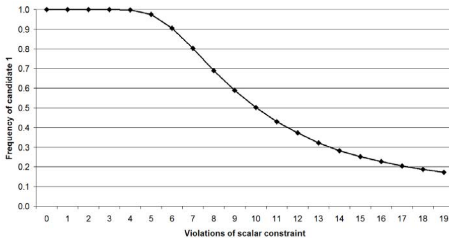
(17) Scalar against constant constraint: sigmoid curve derived under Classical NHG
