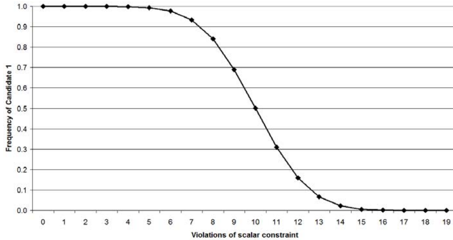
(16) Scalar against constant constraint: sigmoid curve derived under NHG with post-multiplicative noise
