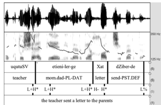
Figure 5: Sample pitch track showing the first element of a compound word “parent”, [eti], receives a pitch accent.
