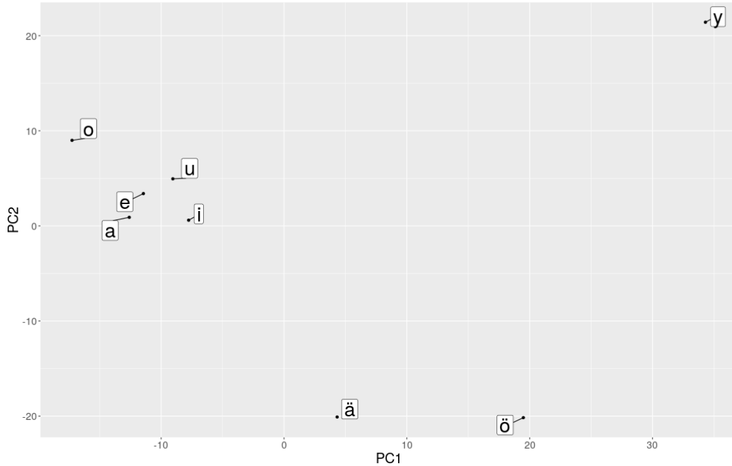
Figure 7.19: A PCA of the vector embedding of vowels from the full Finnish corpus.
