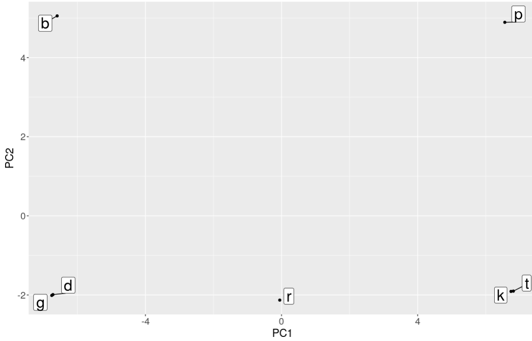
Figure 4.2: A PCA visualization of the vector embedding of Parupa consonants using trigram counts and PPMI weighting.
