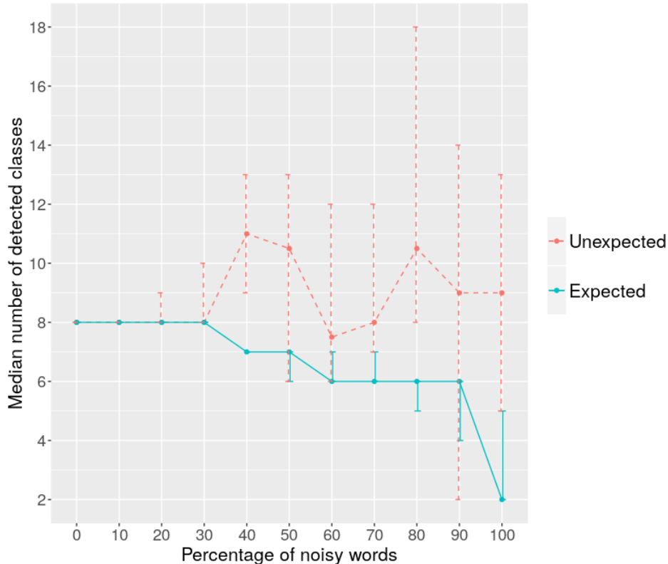
Figure 6.3: A plot of the median number of expected and unexpected classes found by the algorithm as the percentage of noisy words increases. Error bars span the minimum and maximum number of classes retrieved from a corpus at that noise level.
