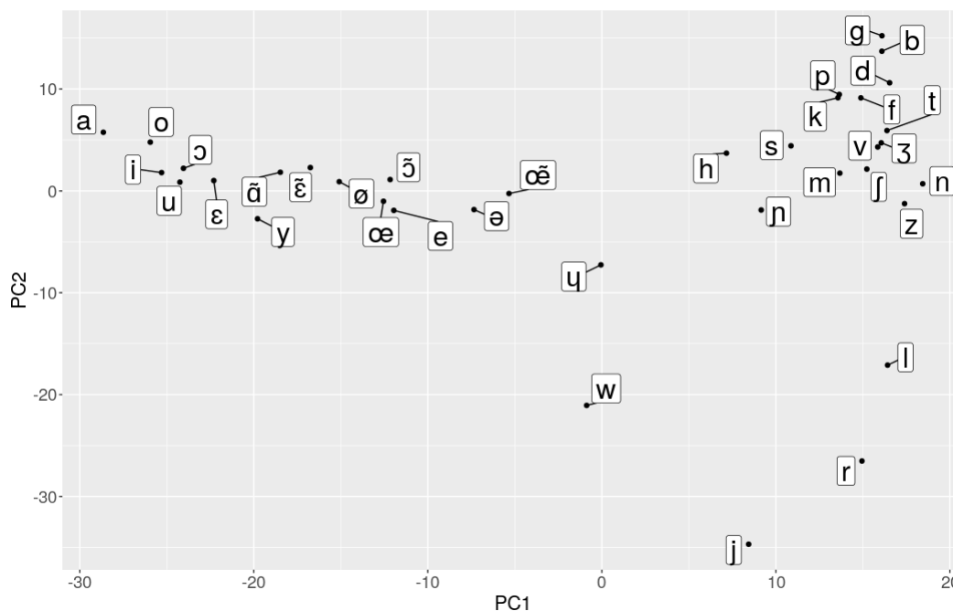
Figure 7.11: A PCA of the vector embedding of French.
