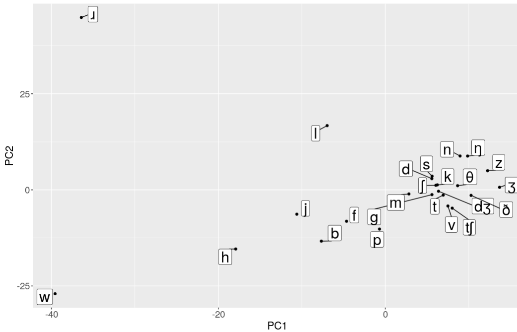
Figure 7.8: A PCA of English consonants.
