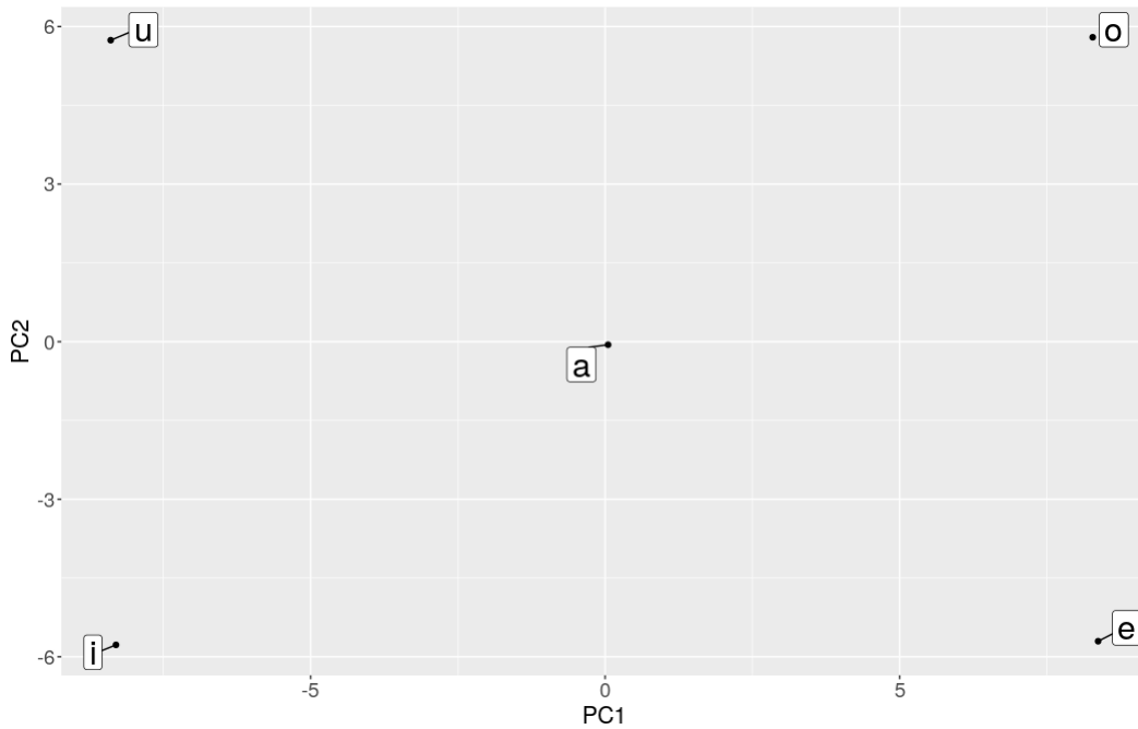
Figure 4.3: A PCA visualization of the vector embedding of Parupa vowels using trigram counts and PPMI weighting.
