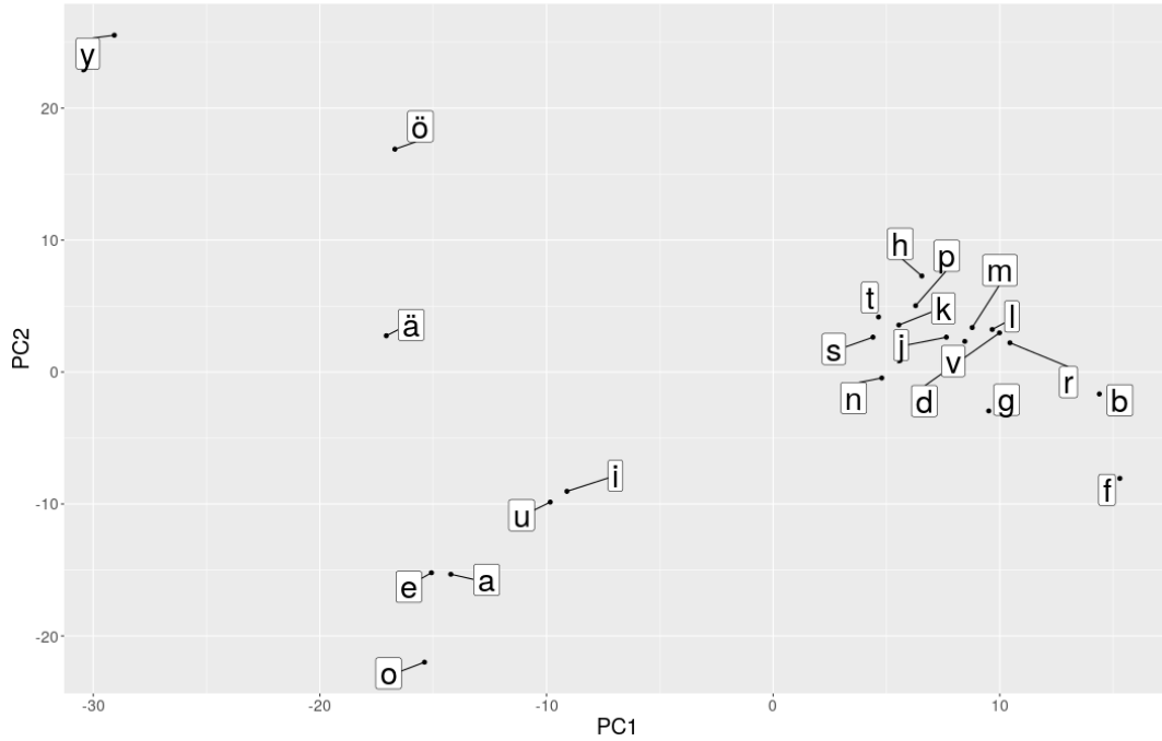
Figure 7.17: A PCA of the vector embedding of the full Finnish corpus.
