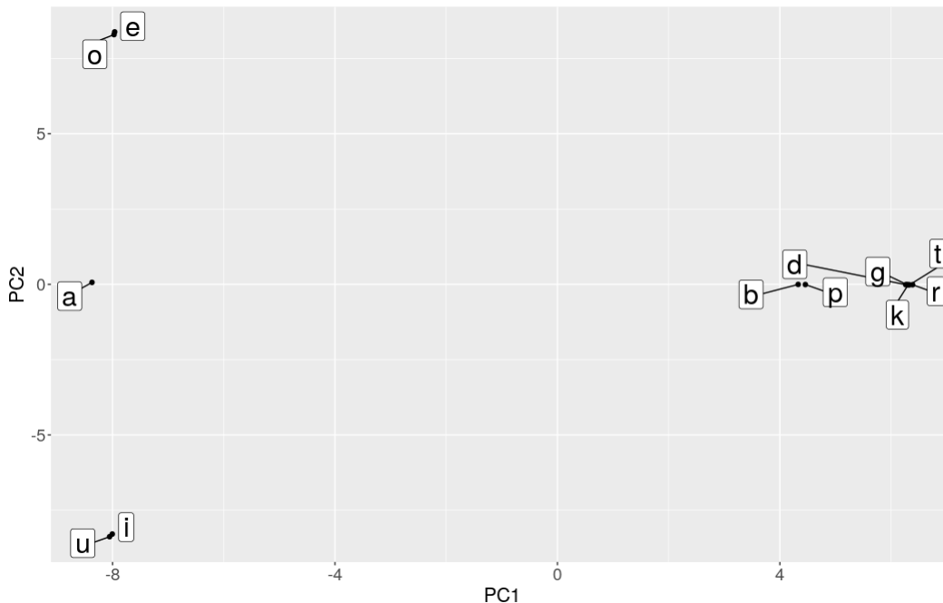
Figure 4.1: A PCA visualization of the vector embedding of Parupa consonants and vowels using trigram counts and PPMI weighting.
